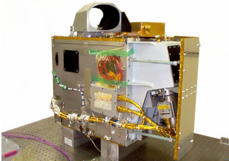
Hyperion Sensor Assembly (HSA)
