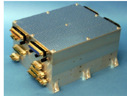
Cryocooler Electronics Assembly (CEA)
